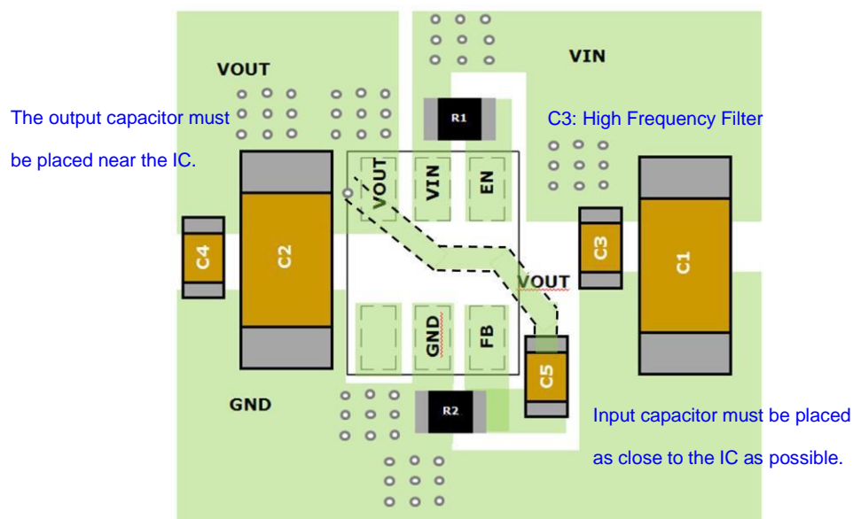
FIG.28 PCB LAYOUT
